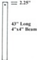
Detail #3 Determining Header Drill Location on Beams
