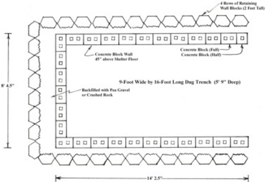
Drawing 2 Supernova Shelter (Top Down View of Shelter Walls)
