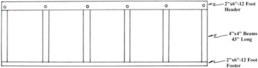
Detail #6 Center Support Structure
